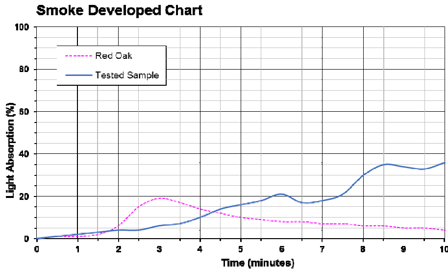
Figure 2 Smoke Developed Chart
