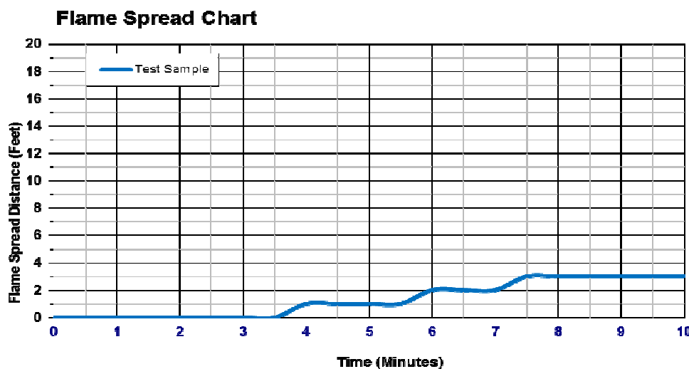
Figure 1 Flame Spread Chart
